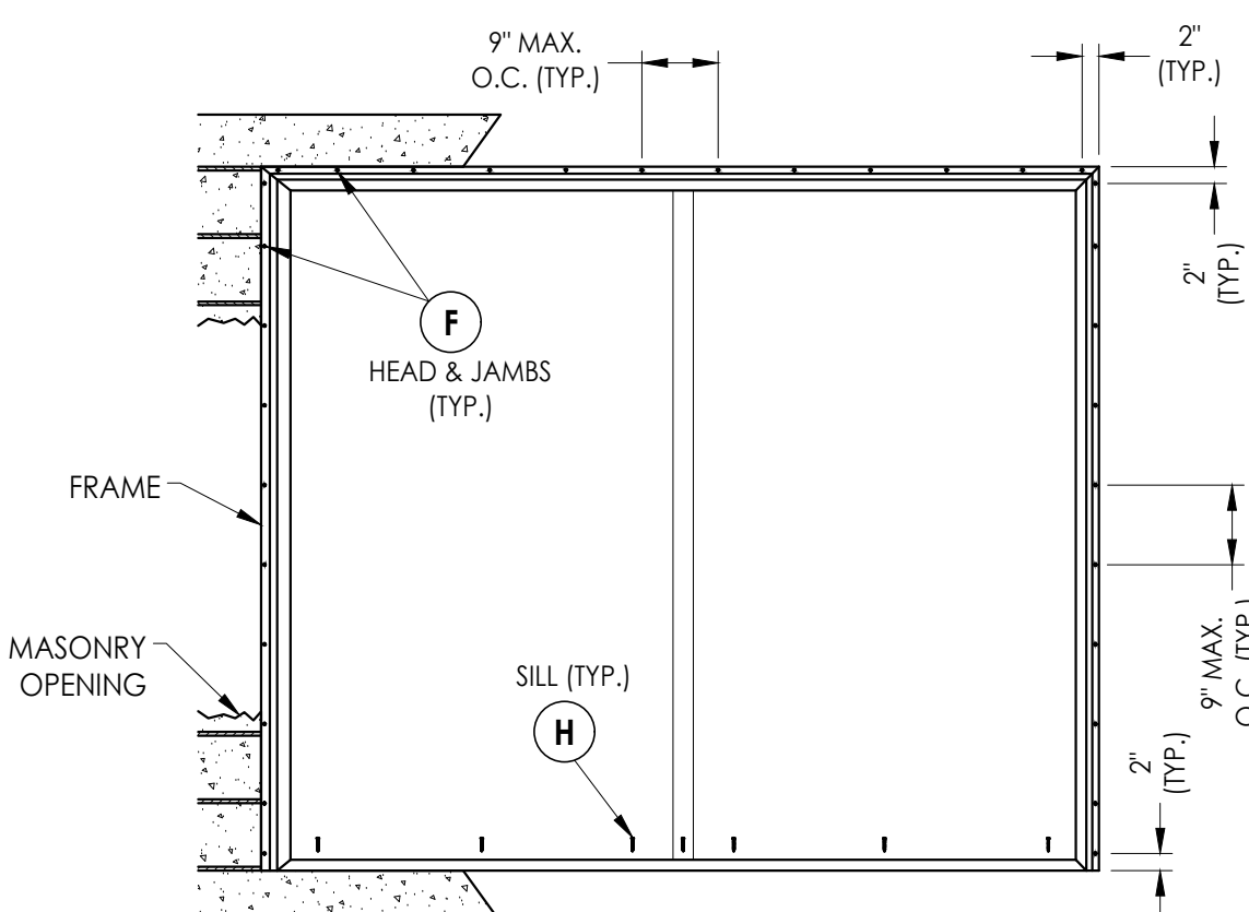
FRAME ANCHORING 2X BUCK
