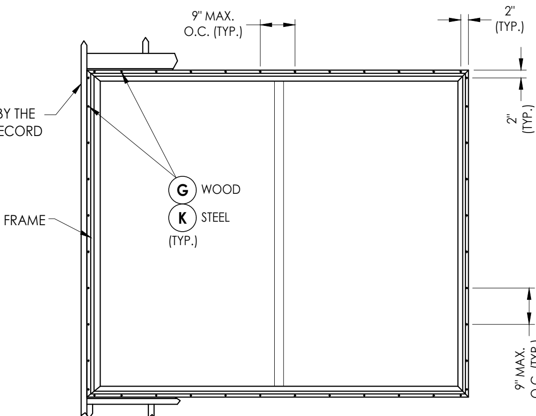
FRAME ANCHORING (2X Stud, Steel Stud)
