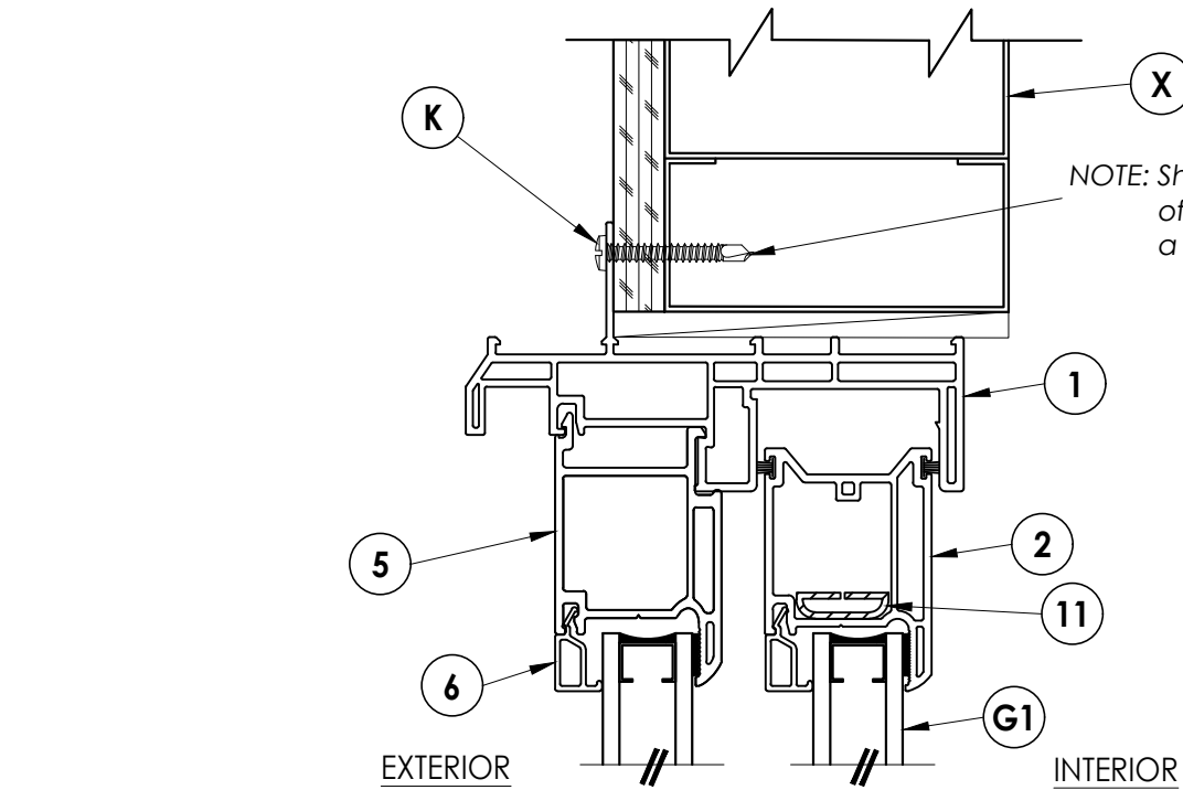
3 3 HORIZONTAL CROSS SECTION Shown w/ Steel Stud framing option
