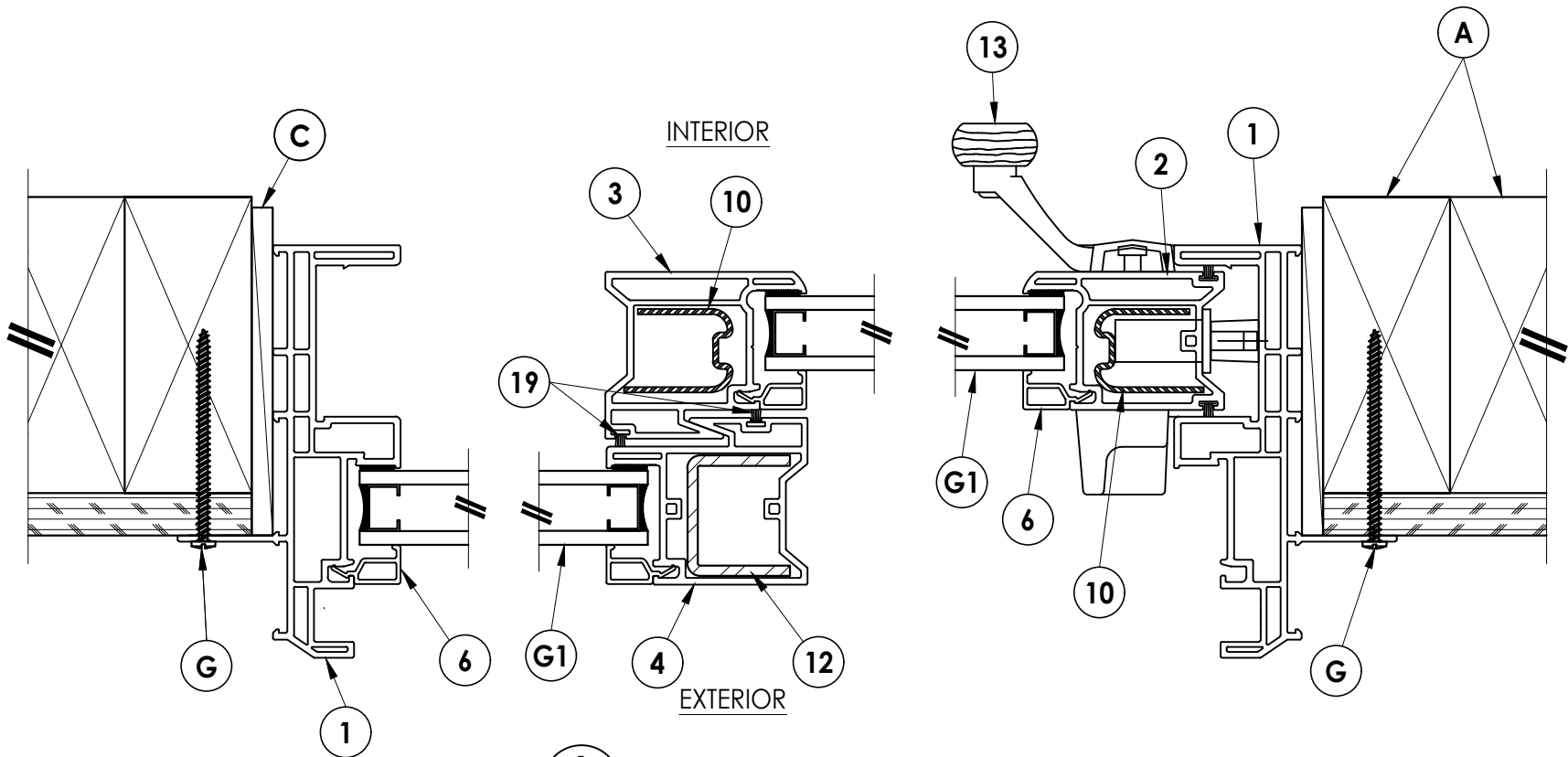
1 3 HORIZONTAL CROSS SECTION Shown w/Stud framing option
